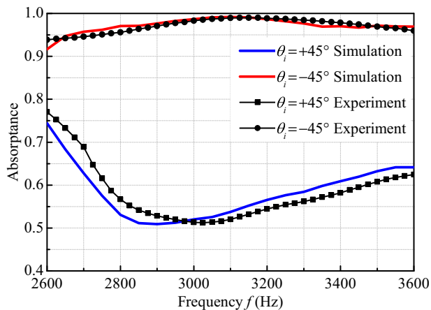
FIG. 7. Numerically calculated and experimentally measured absorbance at different frequencies for opposite incident angles. Blue and red lines represent the simulated absorbances at \theta_i = +45^\circ and \theta_i = -45^\circ , respectively. Black squares and black dots represent the measured absorbance at \theta_i = +45^\circ and \theta_i = -45^\circ , respectively.
